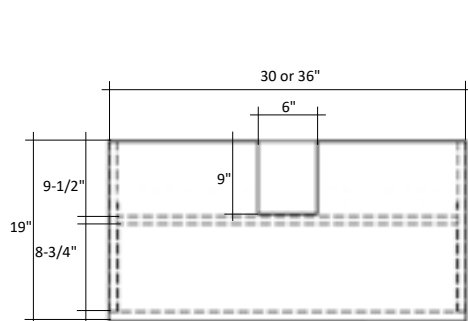
19" Deep Cabinet
