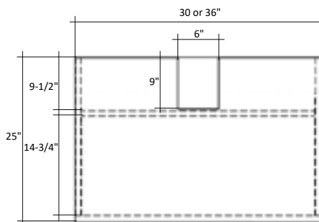
25" Deep Cabinet
