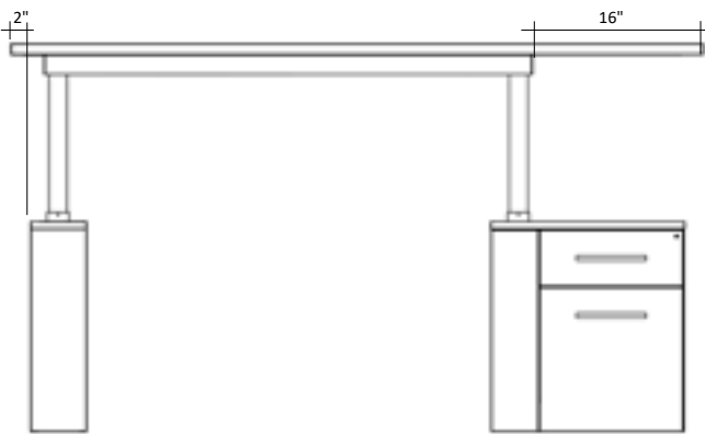
Combination pedestal outset under the worksurface, with over sized worksurface with 16" maximum overhang (Hover Lift Base only).
